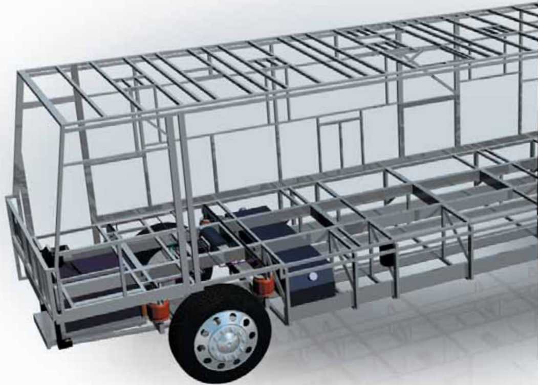
ROADMASTER RR8R-SERIES CHASSIS
